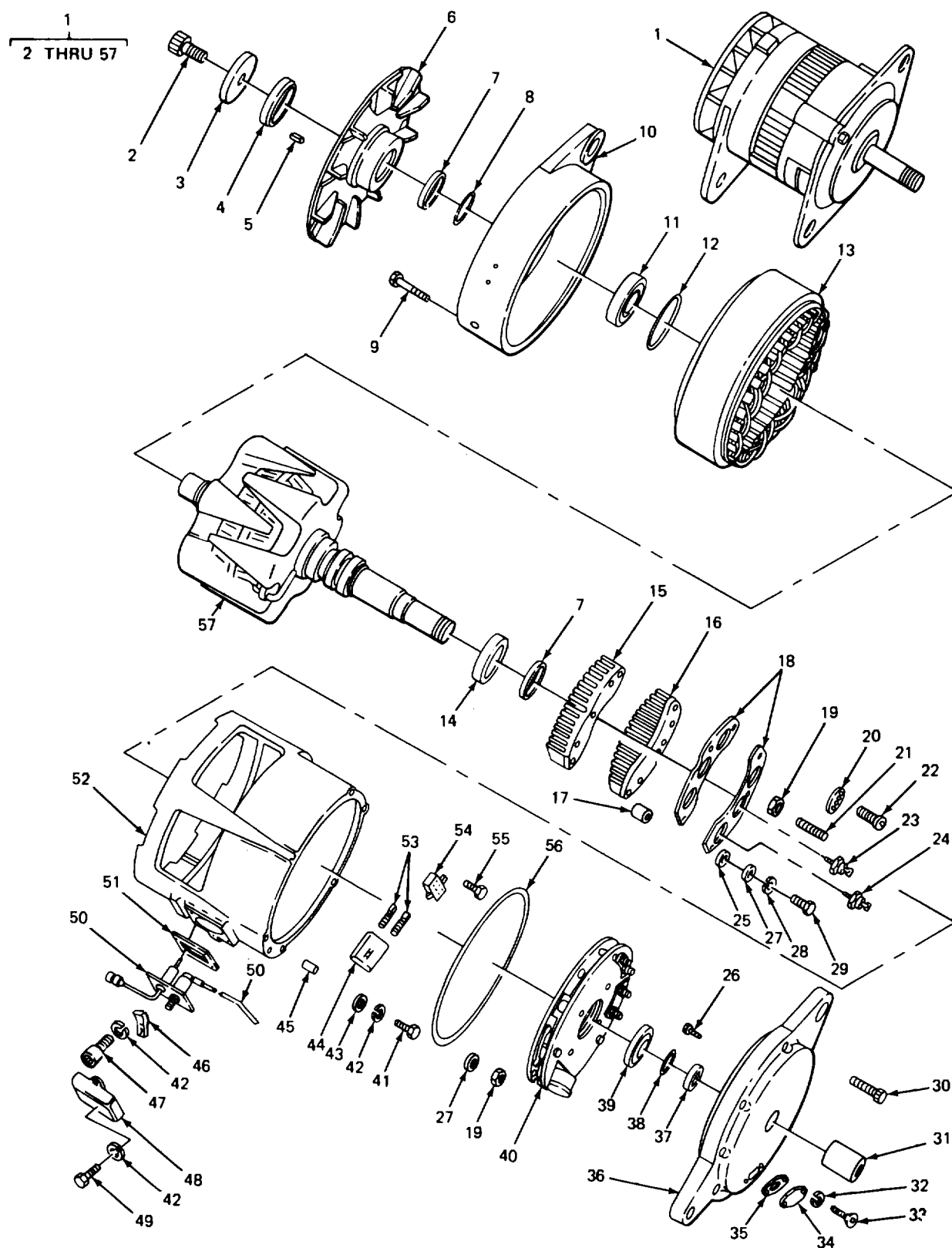
FIGURE 42. ALTERNATOR ASSEMBLY.
