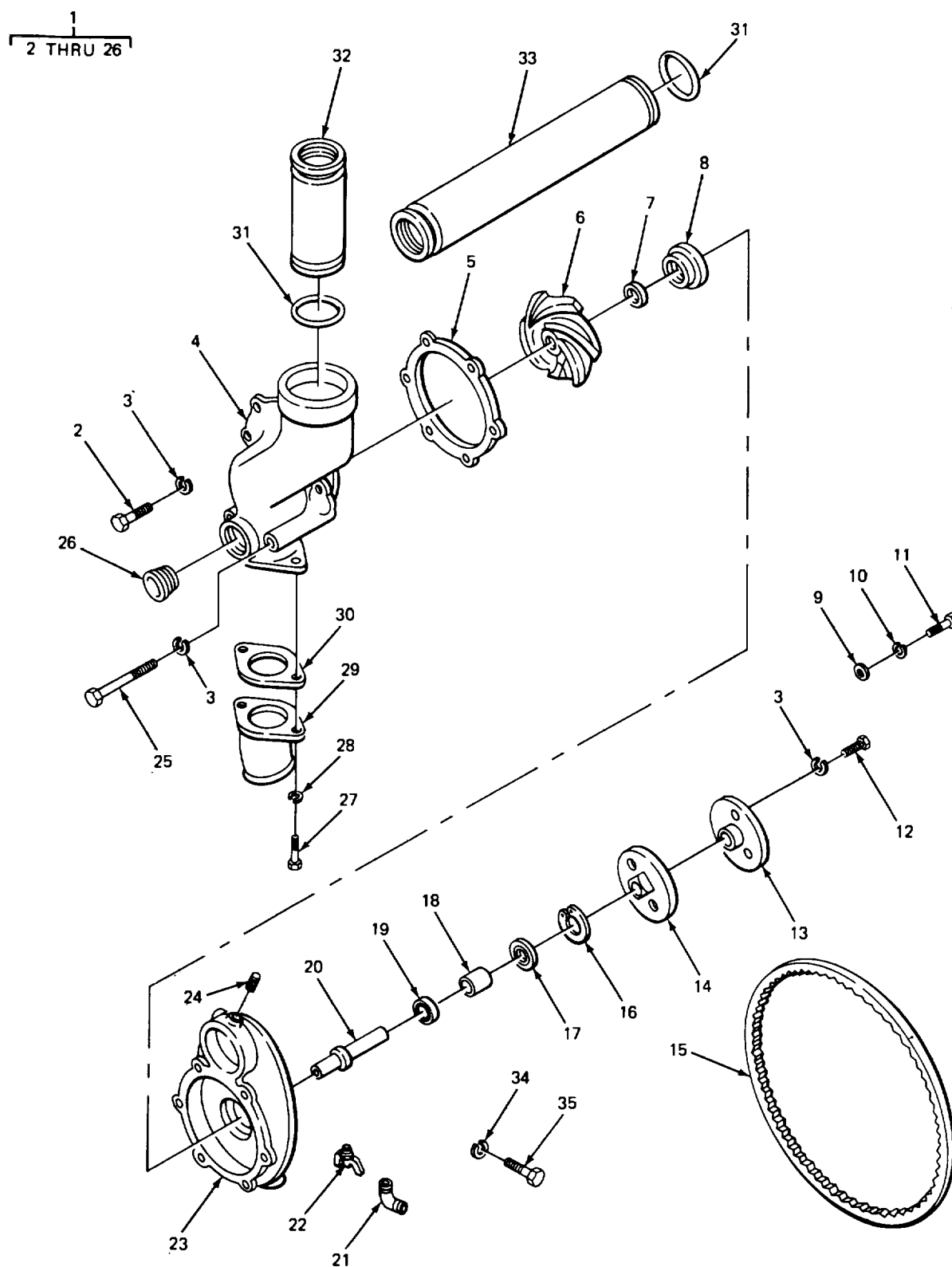
FIGURE 39. WATER PUMP.
