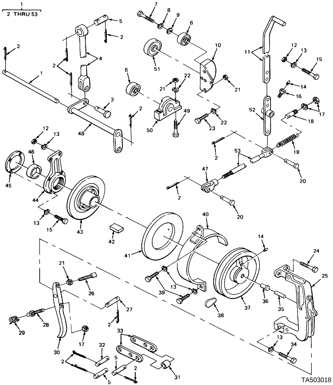
FIGURE 70. DIPPER TRIP.
