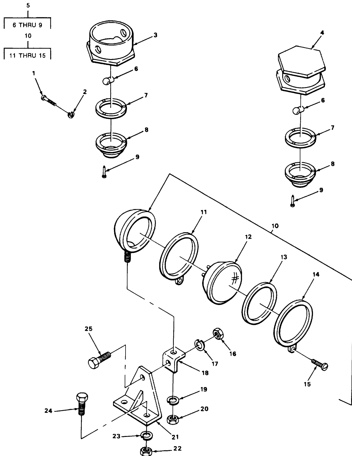
FIGURE 47. LIGHTS.
