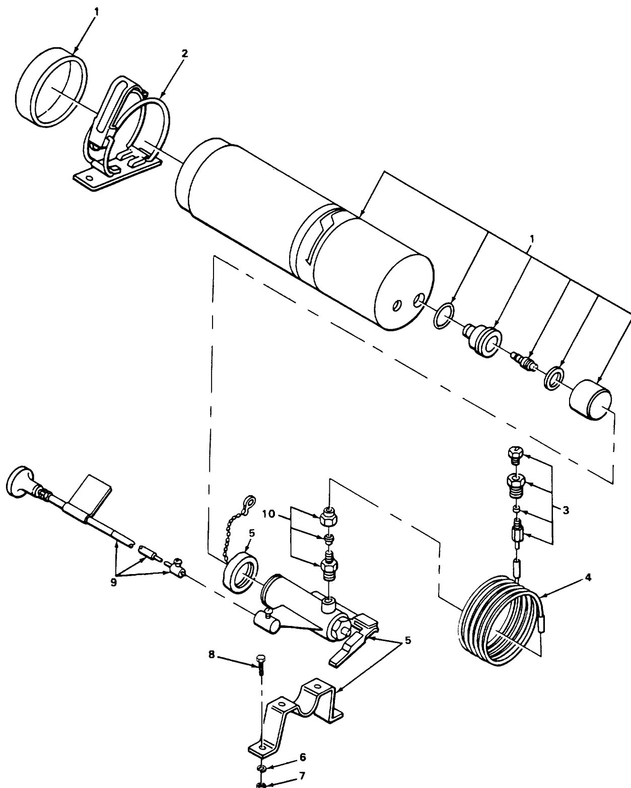
FIGURE 32. ENGINE STARTING AIDS.
