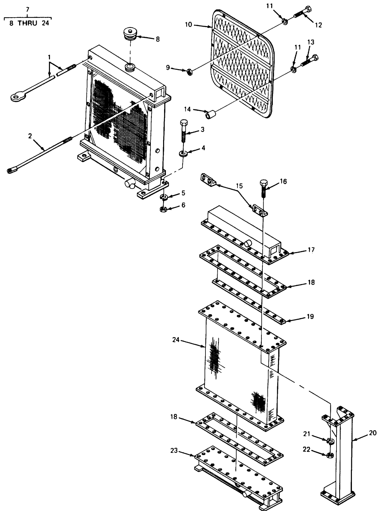
FIGURE 35. RADIATOR.
