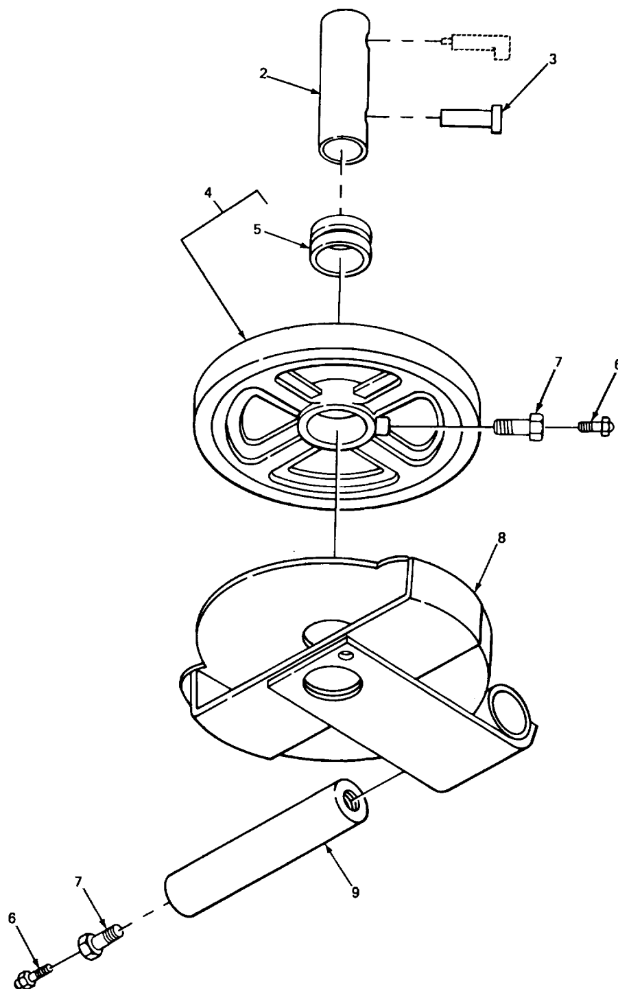
FIGURE 65. SHOVEL PADLOCK
