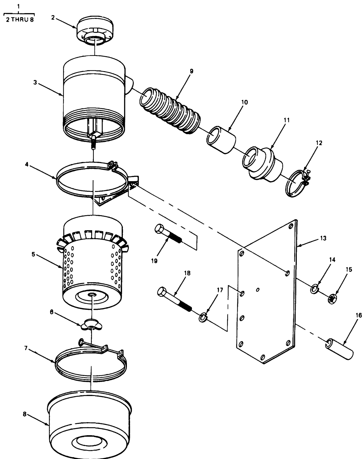
FIGURE 25. AIR CLEANER.
