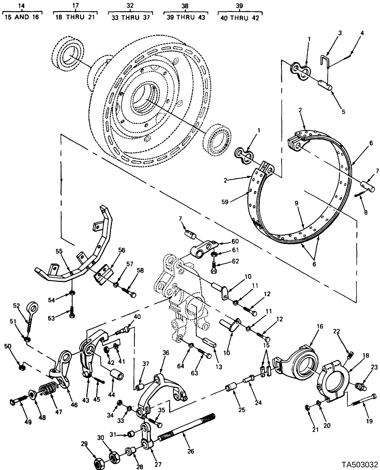
FIGURE 84. CLUTCH ASSEMBLIES
