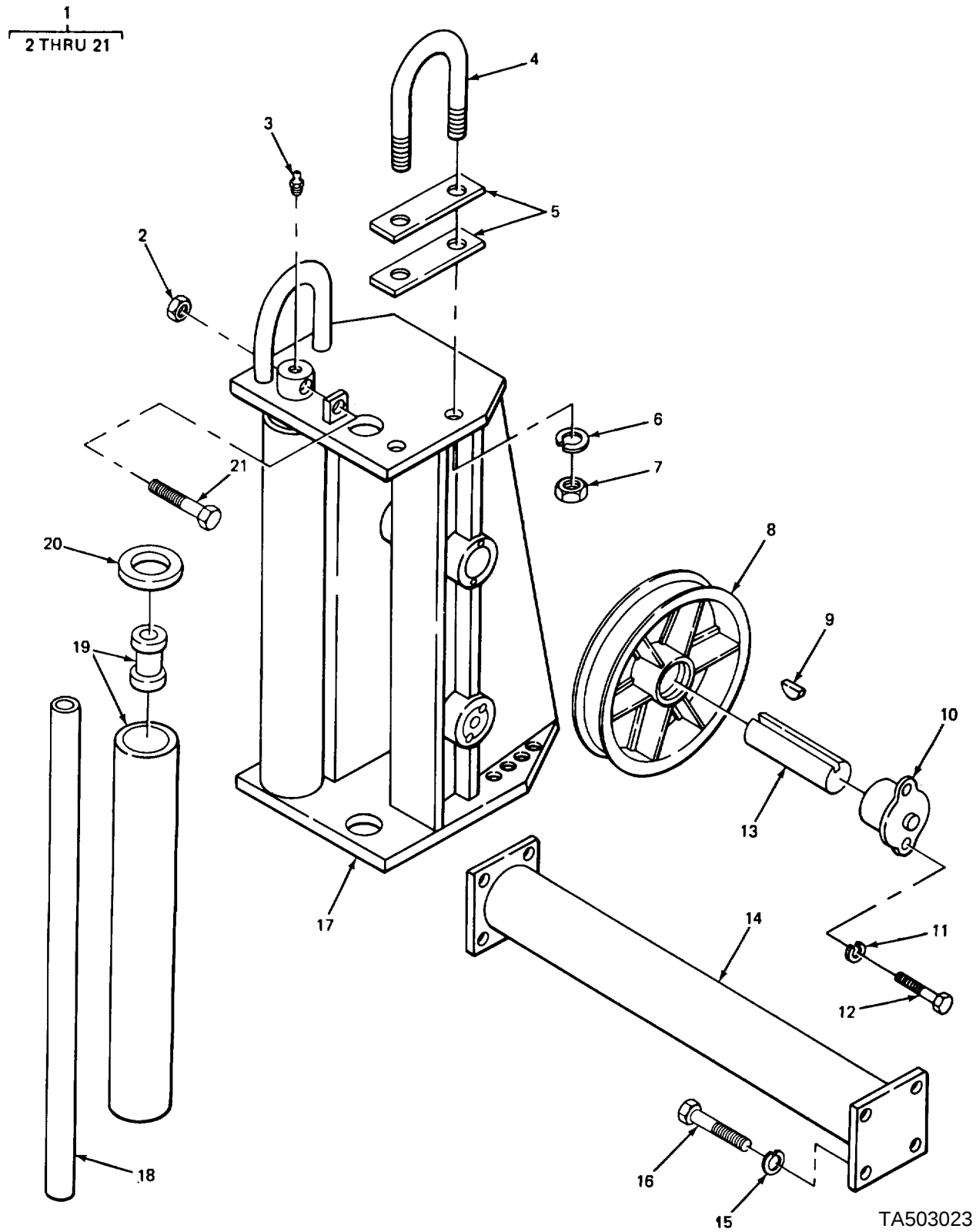
FIGURE 75. FAIRLEAD.
