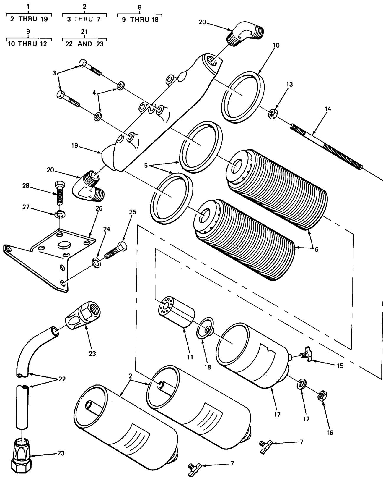
FIGURE 31. FUEL FILTERS.
