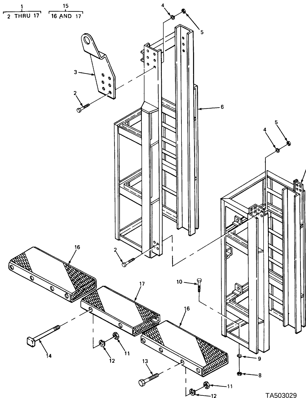
FIGURE 81. PILE DRIVER ASSEMBLY.
