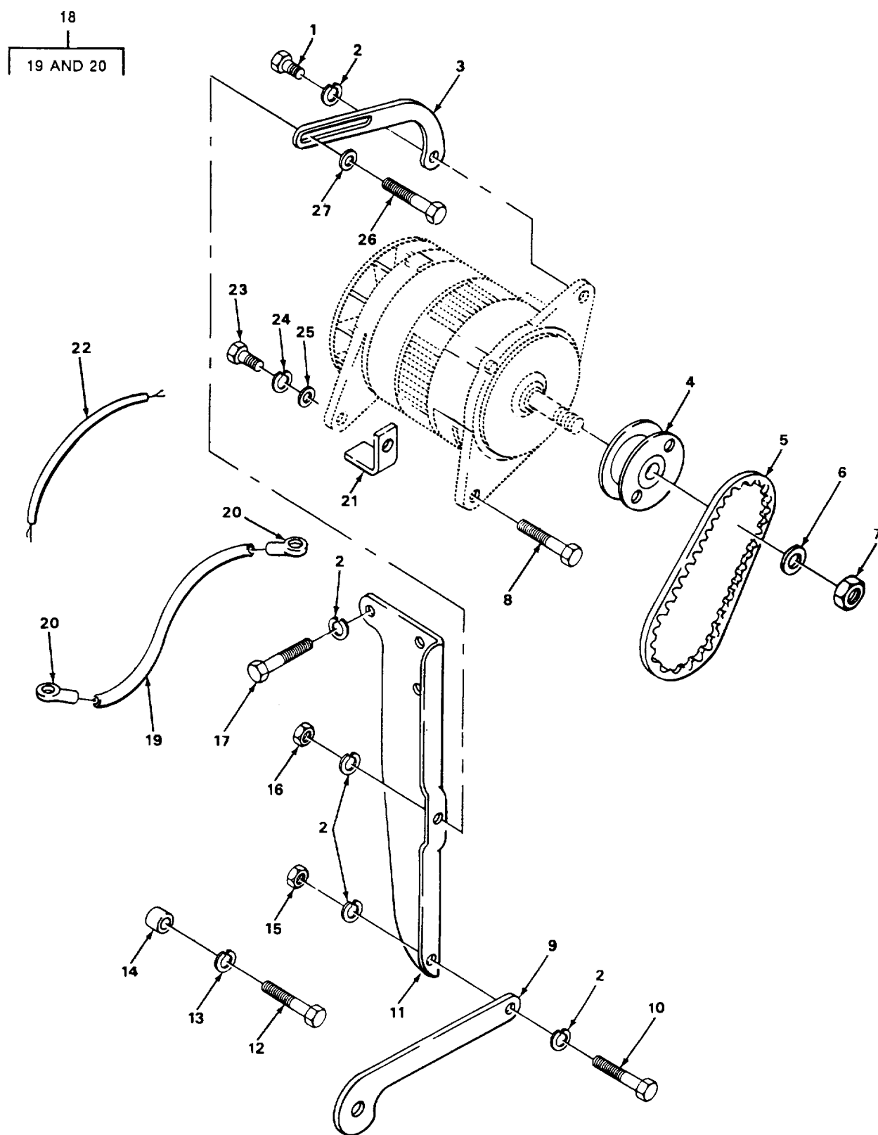
FIGURE 41. ALTERNATOR MOUNTING.
